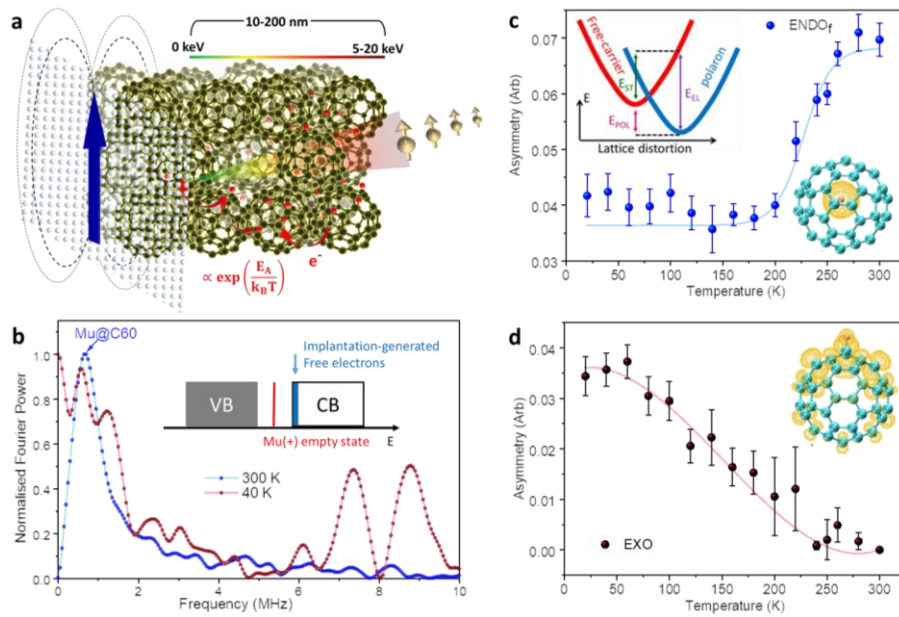
Figure 1. a. Schematic of the ENDO f formation via ionisation, charge hopping and trapping then coupled with molecular rotations. Its oscillation frequency is sensitive to e.g. the electron transfer and emergent magnetism at interfaces. b. Fourier transform of the time domain asymmetry data at ZF for a 210 nm thick amorphous C 60 film on a thermally oxidised Si substrate. The EXO muonium at 1.2, 7.4, and 8.6 MHz is observable at 40 K. At 300 K, only the ENDO f muonium is observed. Inset: ( \sim keV) muon-beam generated free carriers remain delocalized in the conduction band (CB) of the C 60 film, leaving the e-acceptor state of the \mu^+ empty. c. The temperature dependence of the asymmetry attributed to the low-frequency ENDO f together with the calculated spin-density using the PBE exchange-correlation (XC) functional (yellow: 10^{-6} \mu_B \text{ \AA}^{-3} ). A semi-empirical model has been used to fit the temperature dependence leading to an activation energy (equivalent to -E_{POL} ) for ENDO f of E_A = 300 \pm 100 meV.[25] d. Temperature dependence of the EXO signal fraction, also with the calculated PBE spin-density (yellow: 10^{-6} \mu_B \text{ \AA}^{-3} ). The EXO state becomes
